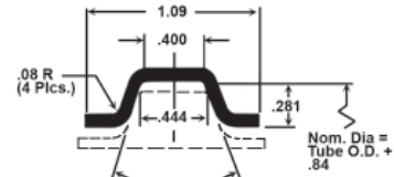
Retainer Gauge: .080 Band Gauge and Width: .063 x 1.000
